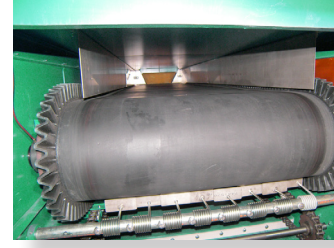
Optional segmented, spring loaded belt scraper
