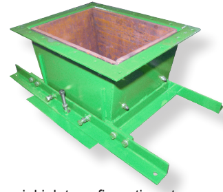
Special inlet configurations to promote material flow and lower motor HP
